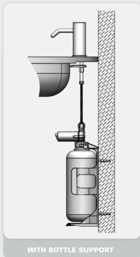
MULTIFEED - TOP FILLING KIT
